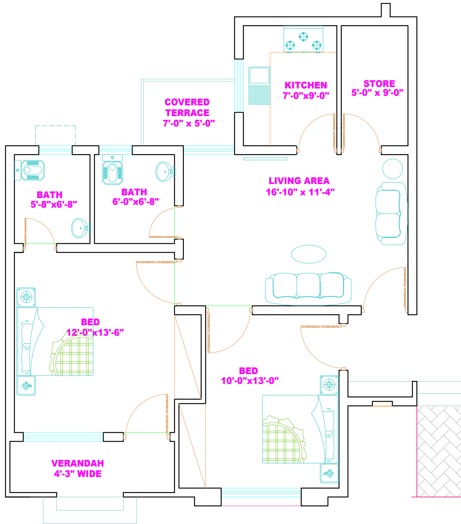
SINGLE UNIT PLAN
